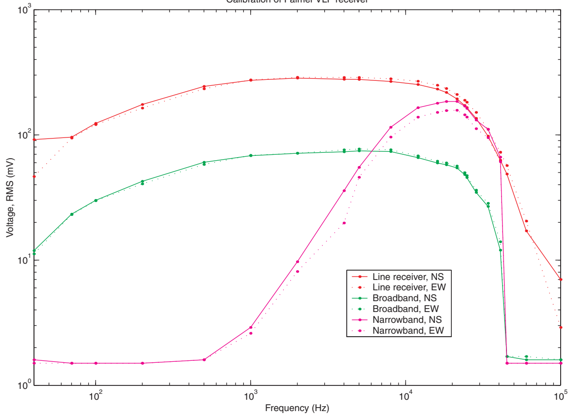
Calibration of Palmer VLF receiver
